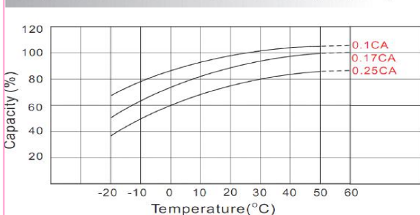
Temperature Effects in Relation to Battery Capacity
